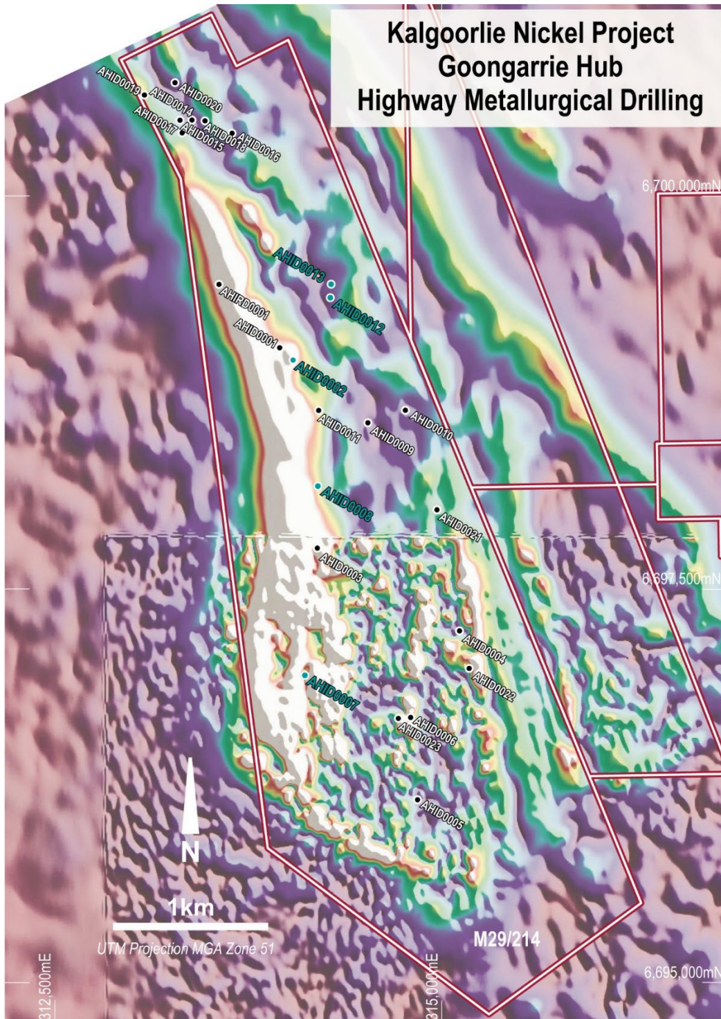
Figure 2: Highway nickel laterite deposit, collar location for Mineralised Neutraliser composites shown as teal color over a 2.5km strike in the Western Accumulate host ultramafic flow, other holes white color. Projection GDA94 MGA94 Zone 51.
